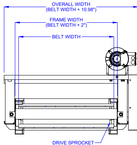
SECTION A-A DRIVE END
