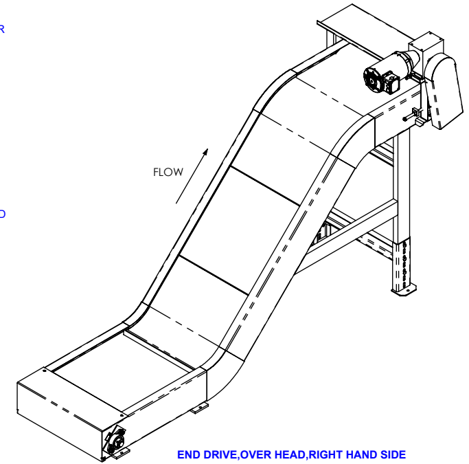
END DRIVE, OVER HEAD, RIGHT HAND SIDE SHBZ - STEEL HINGED BELT CONVEYOR, Z SHAPE
