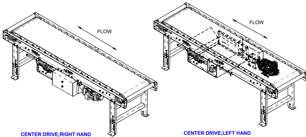
CENTER DRIVE,RIGHT HAND
