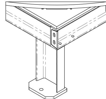
STRUCTURAL CHANNEL WELDED RISERS FOR ELEVATION UP TO 19" (JACK-BOLT SUPPORTS FOR TALLER ELEVATIONS)
