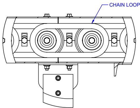
DETAIL C
