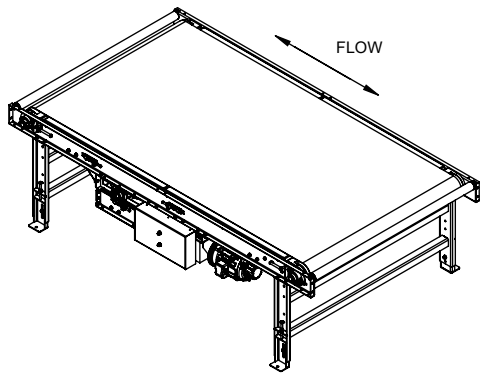
CENTER DRIVE,RIGHT HAND
