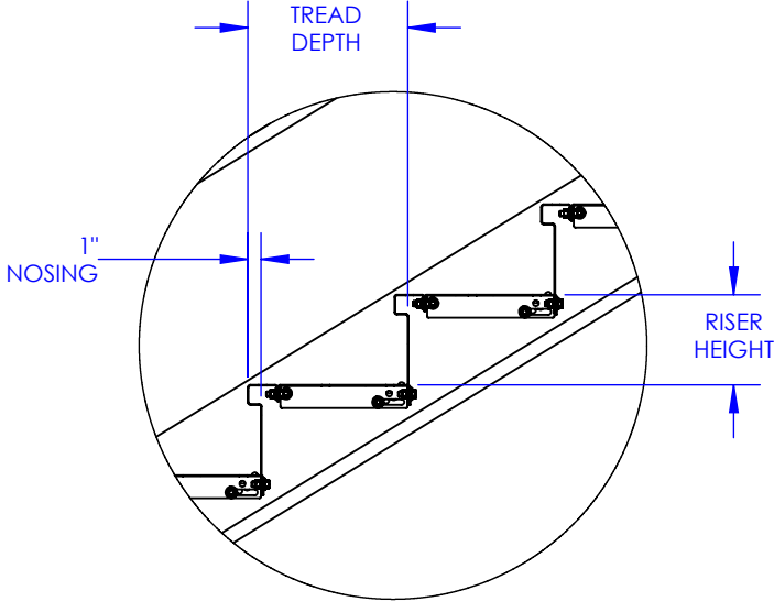
DETAIL F
