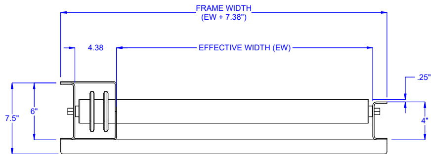
OPTIONAL FRAME FORMED 8 GA. CHANNEL, 6" x 1-1/2" & 4"x 1-1/2"
