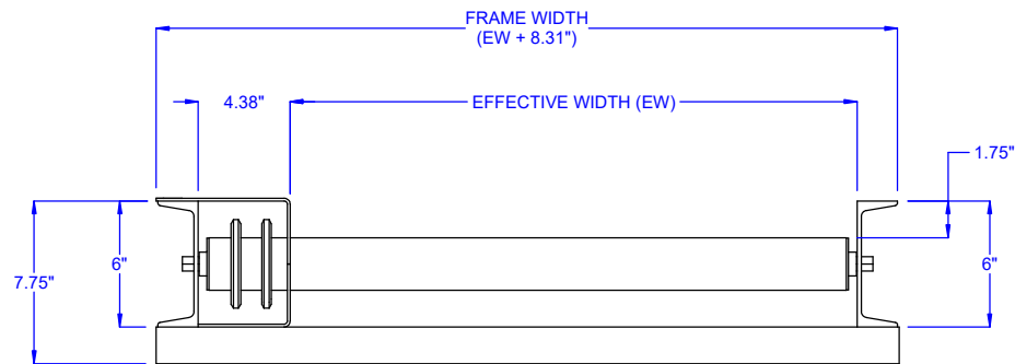
OPTIONAL FRAME STRUCTURAL CHANNEL, 6" x 8.2#
