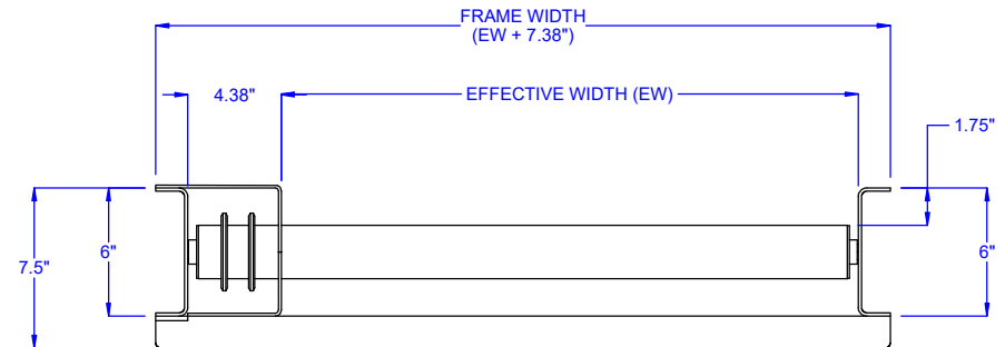
OPTIONAL FRAME FORMED 8 GA. CHANNEL, 6" x 1-1/2"
