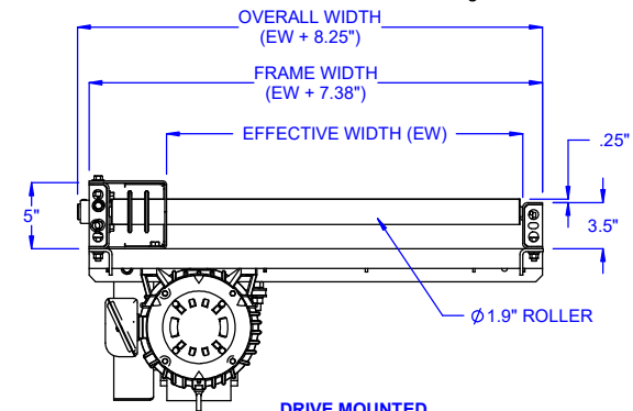
DRIVE MOUNTED BELOW AND WITHIN END VIEW
