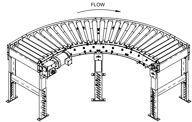
END DRIVE, SIDE, RIGHT, INSIDE RADIUS
