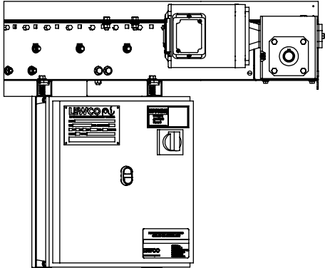
OPTIONAL CONTROLS (COMBINATION MOTOR STARTER OR VFD)
