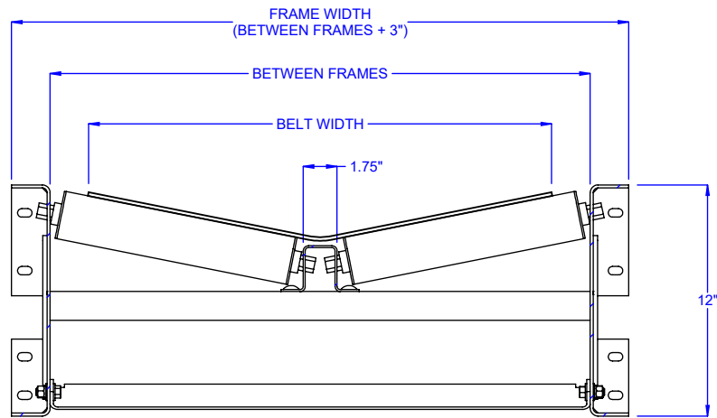
SECTION C-C
