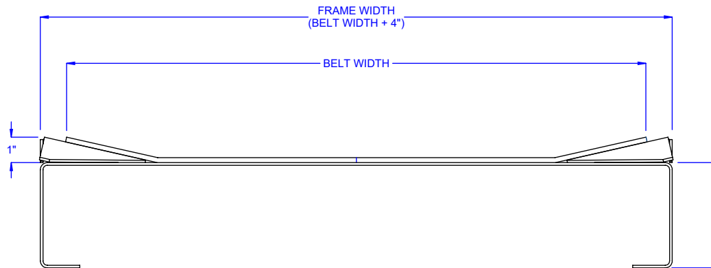
OPTIONAL TROUGH CONSTRUCTION
