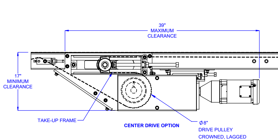
CENTER DRIVE, RIGHT HAND
