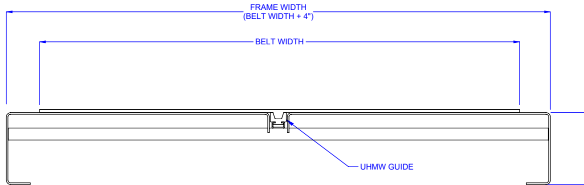
OPTIONAL V-GUIDED CONSTRUCTION (NOTE: PULLEYS ARE GROOVED TO ACCOMMODATE THE V-BELT)
