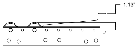
PALLET STOP
