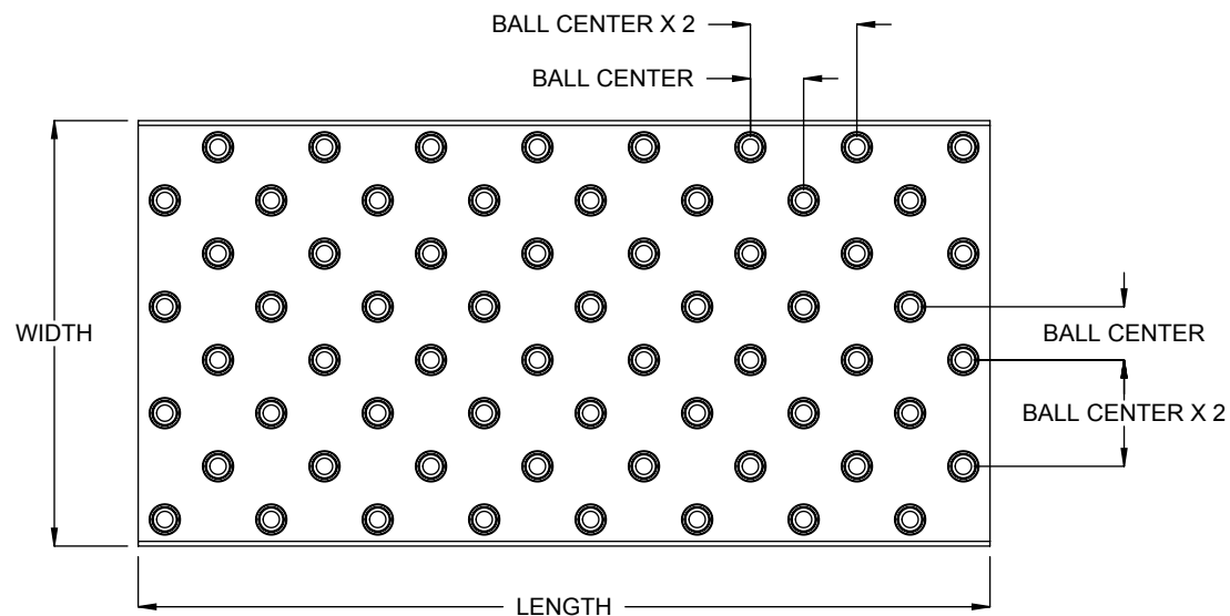
BALL TRANSFER TABLE STYLE B, STAGGERED BALL PATTERN
