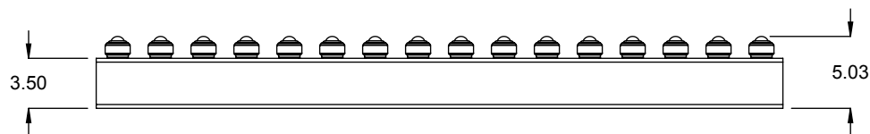
BALL TRANSFER TABLE STYLE B, STAGGERED BALL PATTERN
