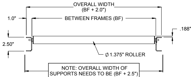
SECTION A-A F98 CHANNEL, 2-1/2" x 1" x 12ga
