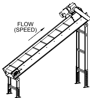
END DRIVE, TOP, RIGHT HAND (SHOWN) END DRIVE, TOP, LEFT HAND (OPPOSITE)
