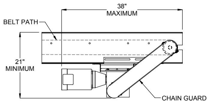
END DRIVE, BOTTOM
