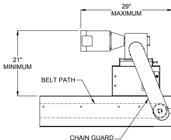
END DRIVE, TOP
