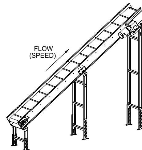
END DRIVE, SIDE, RIGHT HAND (SHOWN) END DRIVE, SIDE, LEFT HAND (OPPOSITE)
