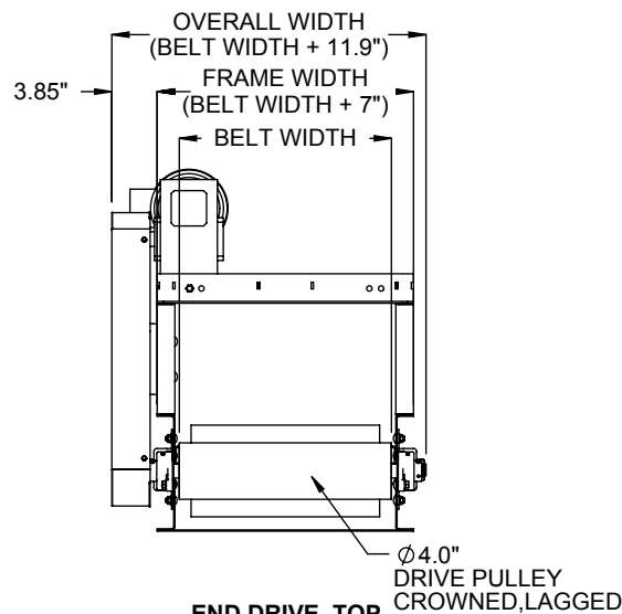
END DRIVE, TOP END VIEW
