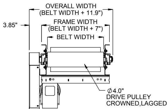
END DRIVE, BOTTOM END VIEW
