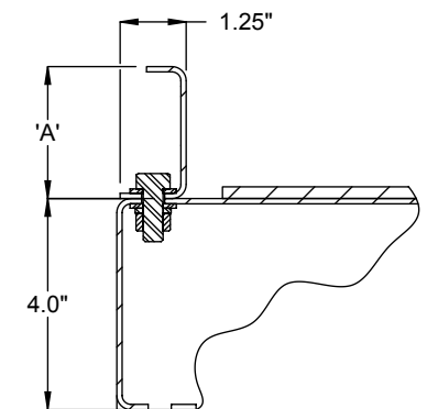
12ga BOLT ON CHANNEL
