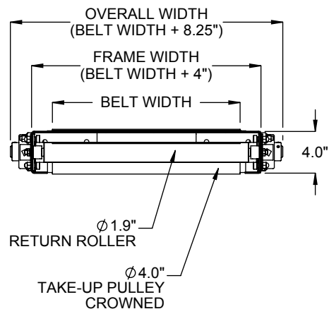
SECTION A-A TAKE-UP END TYPICAL ALL DRIVES
